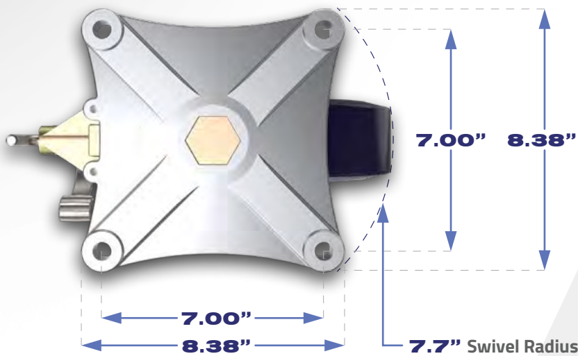
Four Mounting Holes for 1/2" Diameter Bolts.
