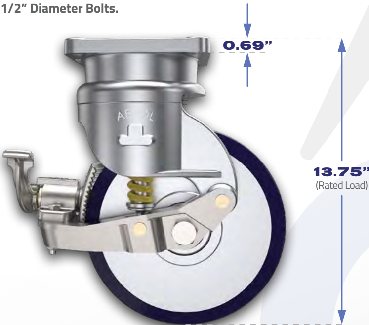
Four Mounting Holes for 1/2" Diameter Bolts.
