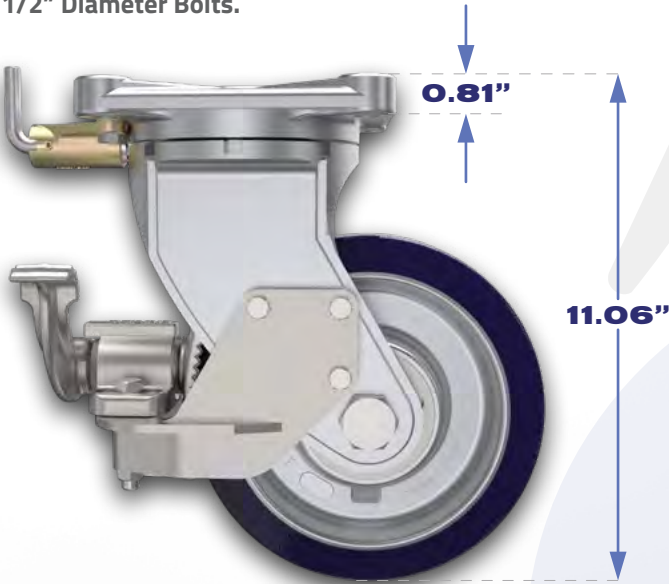
Four Mounting Holes for 1/2" Diameter Bolts.
