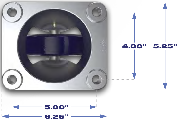
Four Mounting Holes for 1/2" Diameter Bolts.
