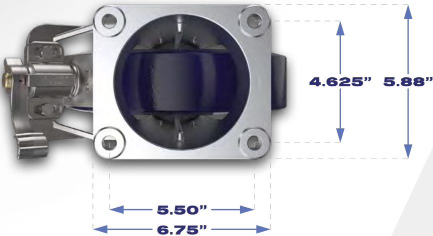
Four Mounting Holes for 1/2" Diameter Bolts.
