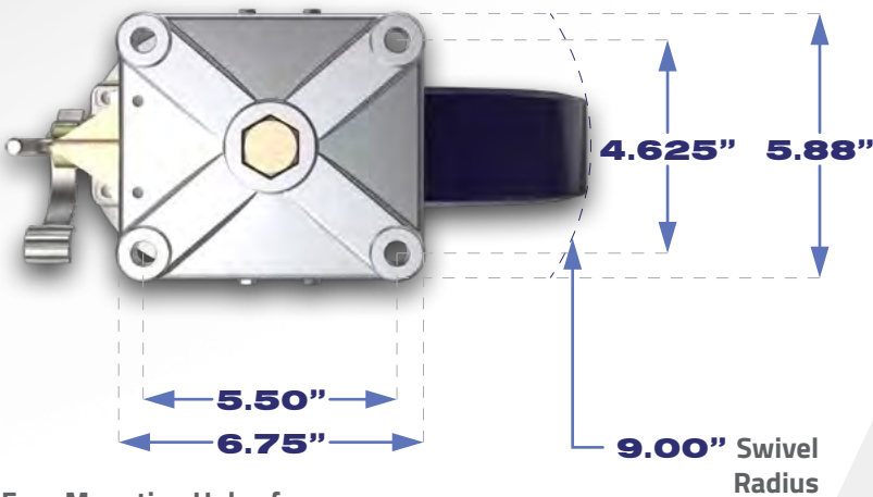
Four Mounting Holes for 1/2" Diameter Bolts.
