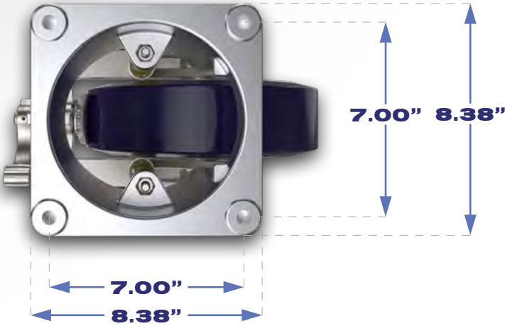
Four Mounting Holes for 1/2" Diameter Bolts.
