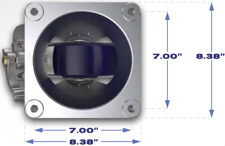
Four Mounting Holes for 1/2" Diameter Bolts.
