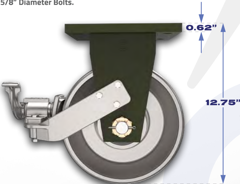
Four Mounting Holes for 5/8" Diameter Bolts.
