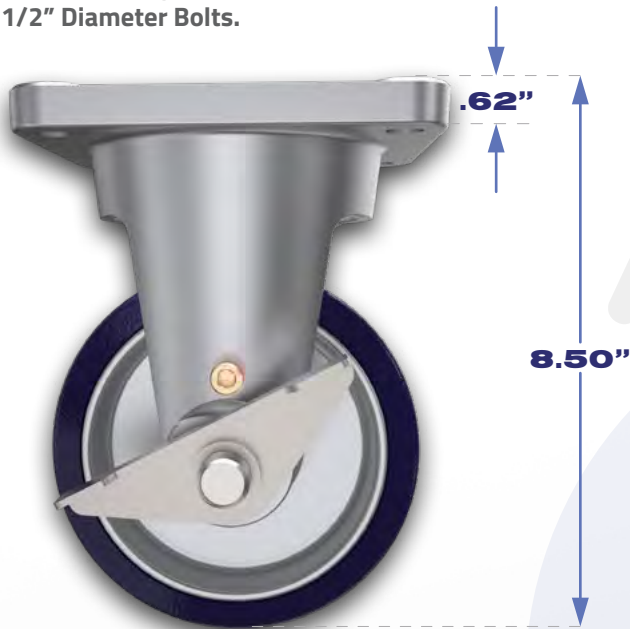
Four Mounting Holes for 1/2" Diameter Bolts.
