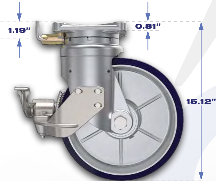
Four Mounting Holes for 1/2" Diameter Bolts.
